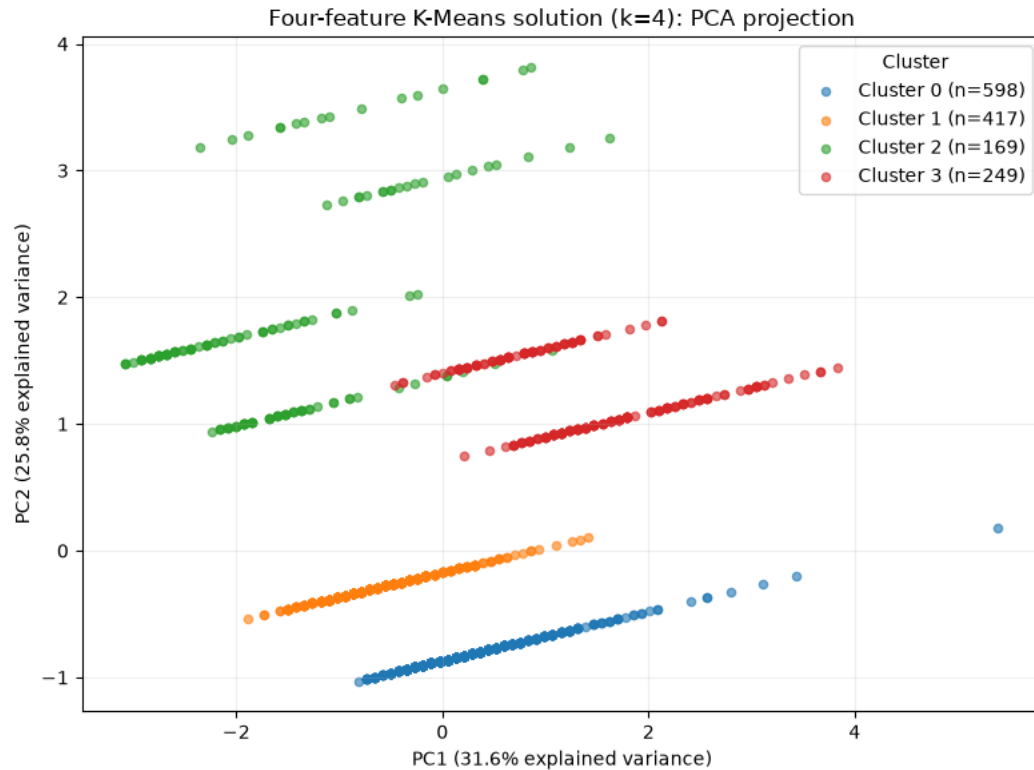
Figure 2: PCA projection of the age-corrected four-feature K-Means solution ( k = 4 ). Colours indicate cluster membership. The two components explain 57.32% of the total variance.
